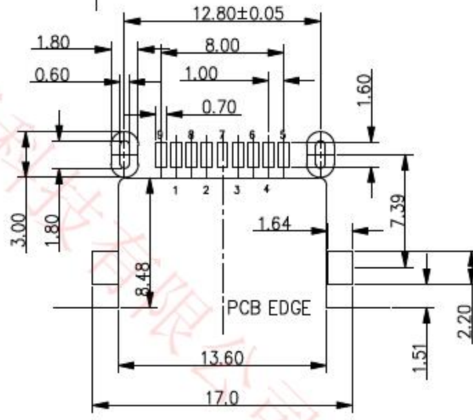
RECOMMENDED PCBA LAYOUT (TOLERANCE+±0.05)
