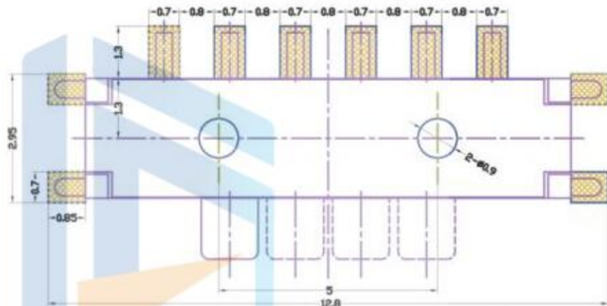
P.C.B MOUNTING PATTERN DIMENSION
