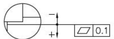
A DETAIL COPLANARITY
