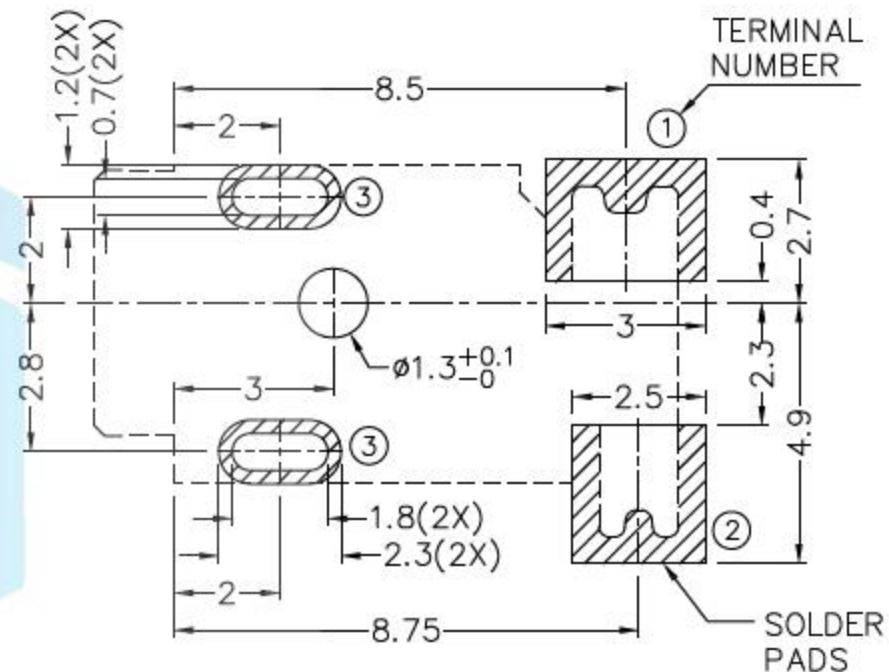
RECOMMENDED P.C.B. LAYOUT TOLERANCE: ±0.05 (TOP VIEW)
