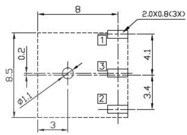
RECOMMENDED P.C.B. LAYOUT UNSPECIFIED TOLERANCE ±0.05 (BOTTOM VIEW)
