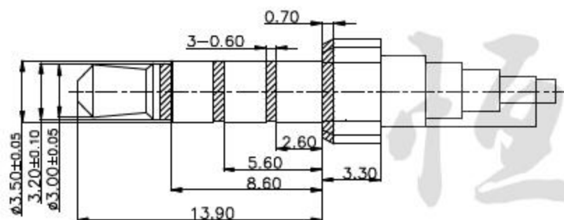
Ø3.5 5POLE PLUG
