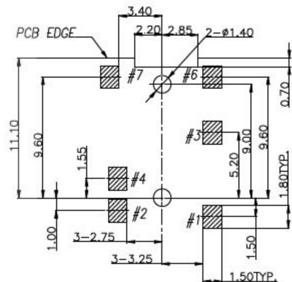
P.C.B LAYOUT MOUNTING PATTERN (TOP VIEW)
