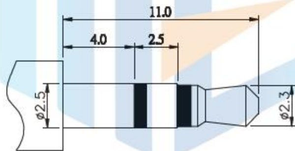
φ2.50mm 3 POLE PLUG
