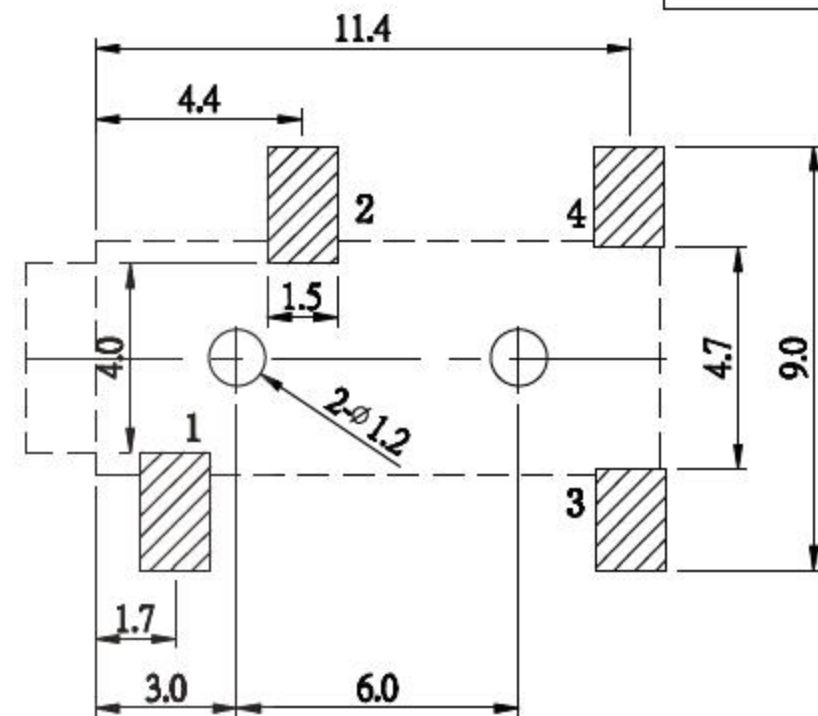
P.C.B LAYOUT MOUNTING PATTERN (TOP VIEW)
